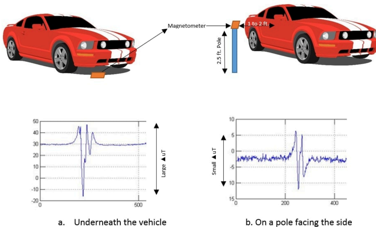
Figure 1 Sensor Placements
